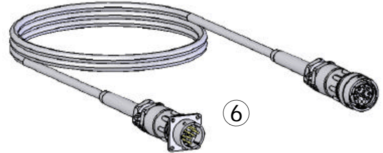
JSHK5-E 5m extension cable, between (for instance) JSHK10 and JSHD4.
