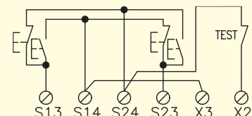
Emergency stop with manual resetting.
