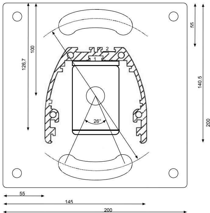
fig 24/2 column assembled with light curtain ULVT/BLVT
