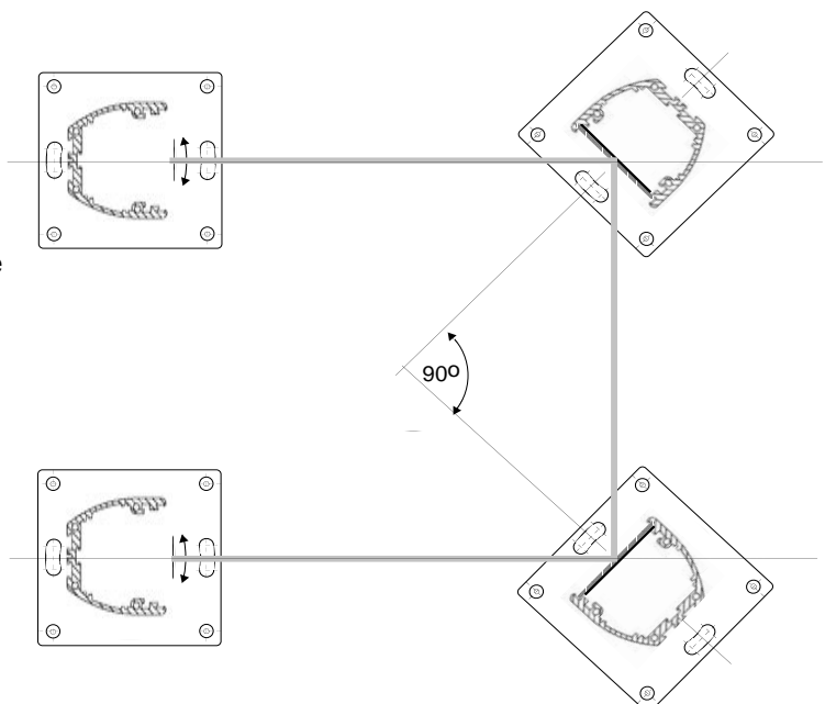
fig 23/4 Installation of the columns
