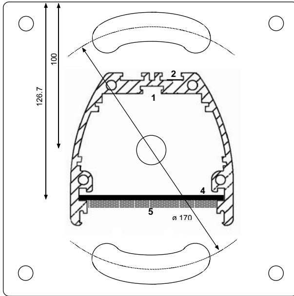
fig 24/1 column with tilted mirror
