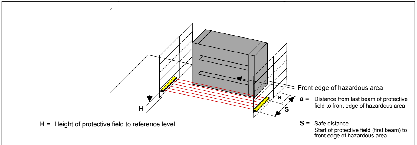
fig 15/1 Horizontal protection
