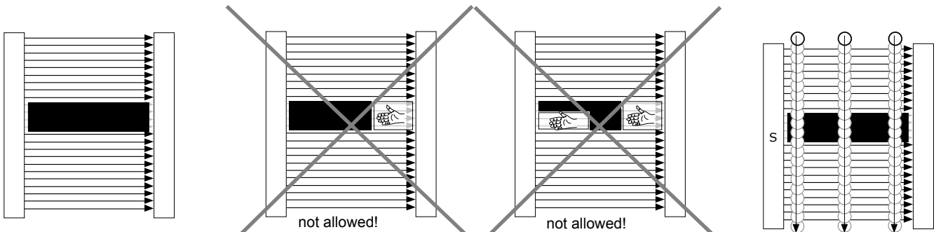
fig 29.1 Fixed Blanking or Floating Blanking with full utilization of the blanked sector of the light curtain.
