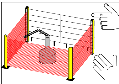
Fig. 4/4: Barricading of access areas by means of deflecting mirrors
