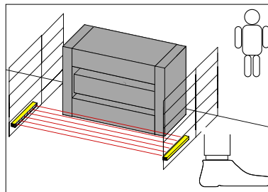
Fig. 4/2: Barricading of sectors
