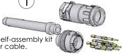
JSHK0 Self-assembly kit (female) for cable.
