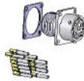
JSHK1-A Self assembly kit (female) for use with JSHK5-E1, on machine.
